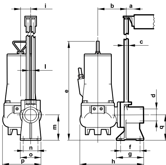
Fig. 17 Series GRINDER - FEKA 2500
