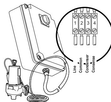
Fig. 9 Low tension connection scheme
