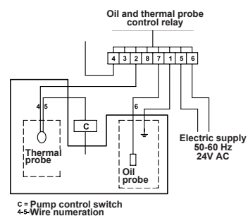
Fig. 13 Thermal probe connection
